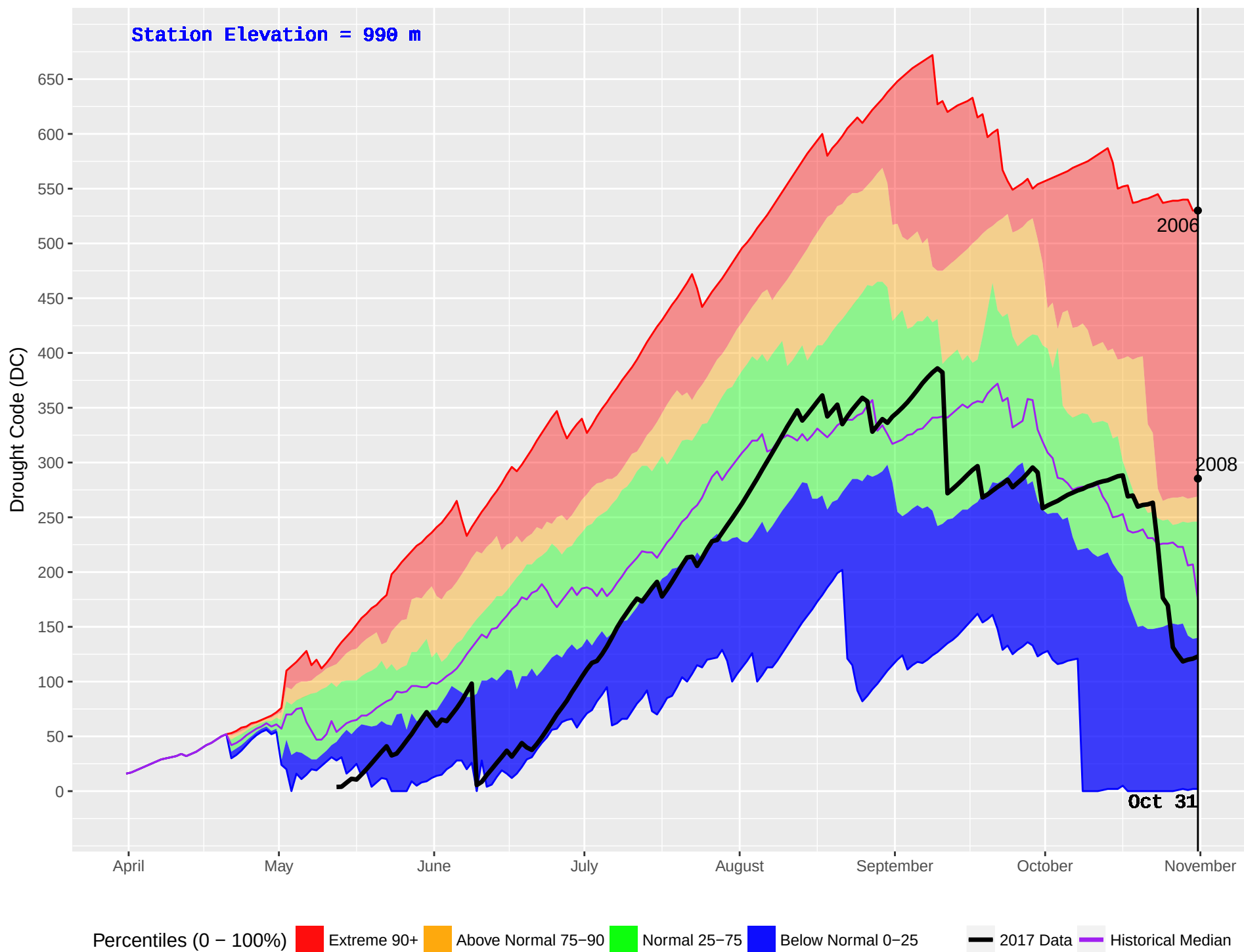
LOVELL COVE (163) : Historical (1979–2016) and Current (2017) Noon Drought Code (DC)
