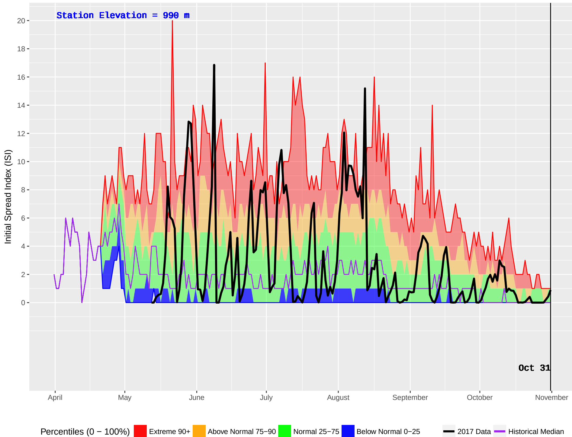
LOVELL COVE (163) : Historical (1979–2016) and Current (2017) Noon Initial Spread Index (ISI)
