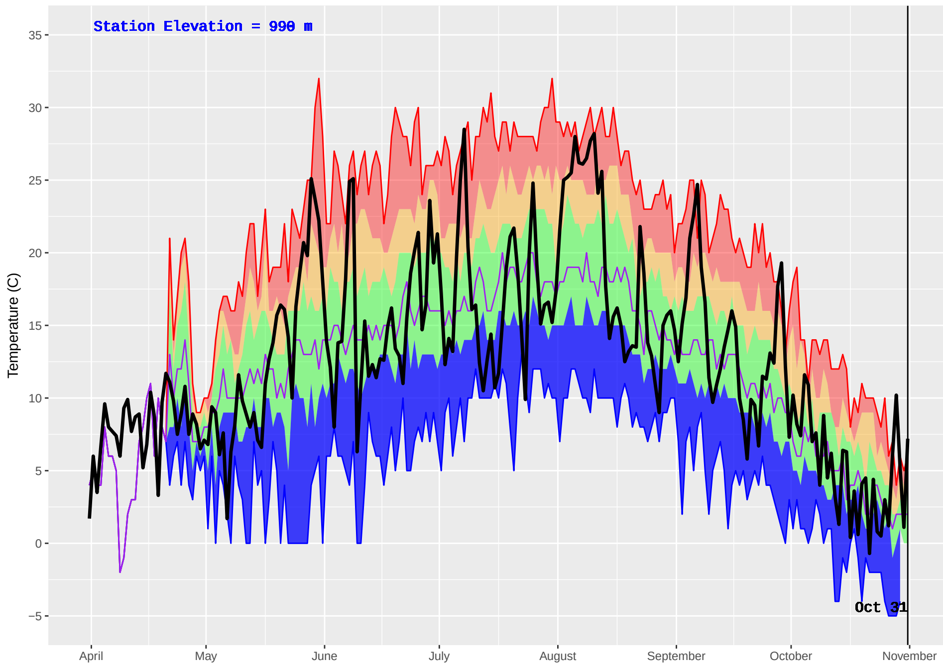
LOVELL COVE (163) : Historical (1979–2016) and Current (2017) Noon Temperature
