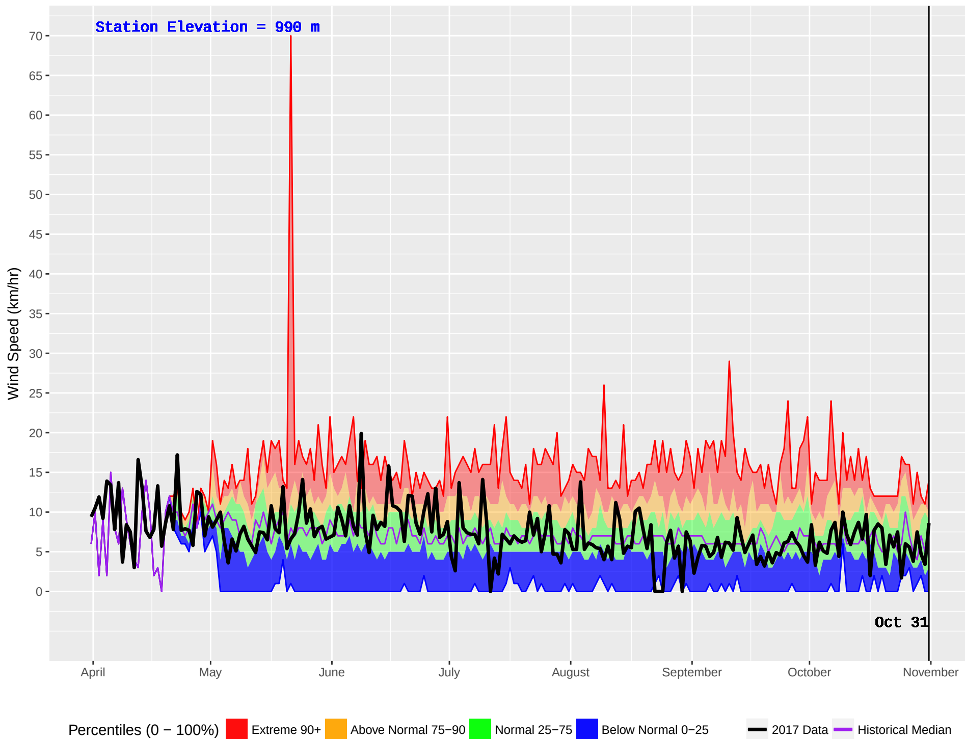
LOVELL COVE (163) : Historical (1979–2016) and Current (2017) Noon Wind Speed
