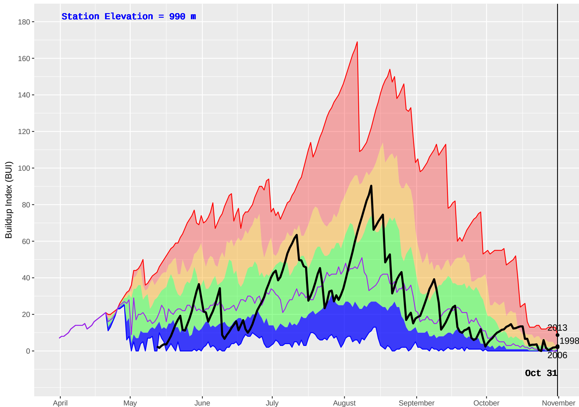
LOVELL COVE (163) : Historical (1979–2016) and Current (2017) Noon Buildup Index (BUI)
